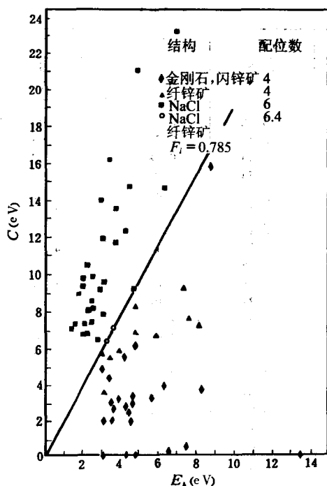
图 2-6 AN^B-N 晶体的 E_g 和 C 值 f_i = 0.785 线把四配位和六配位晶体分开 数据摘自: J. C. Phillips, Bonds and Bands in Semiconductors p42, Academic press New York and London(1973).
